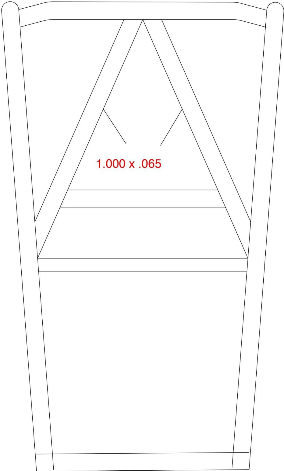
Midget Frame Dimensions
