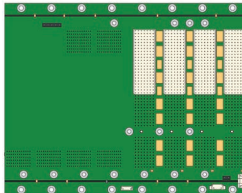
CompactPCI Plus I/O 3 U Rear view
