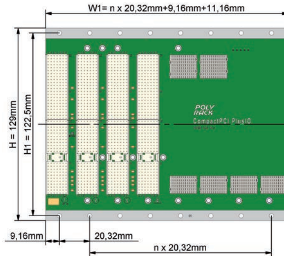
Dimension diagrams
