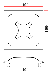
⑮ BOTTOM PANEL (1X1) Model no. 1-1-B
