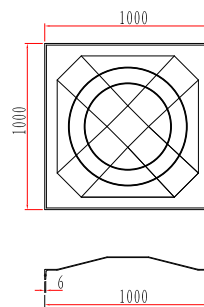
⑬ ROOF PANEL (1X1) Model no. 1-1-T
