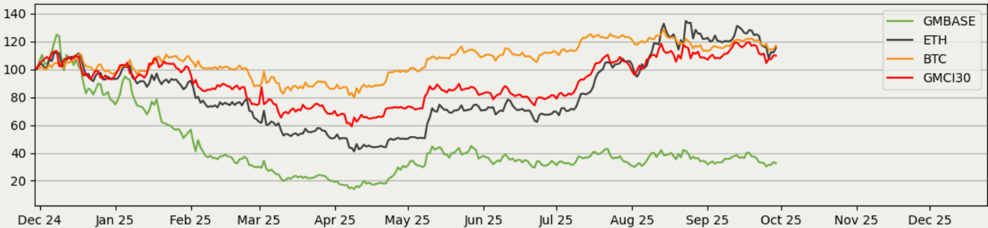
Performance GMBASE vs GMCI30 vs BTC vs ETH
