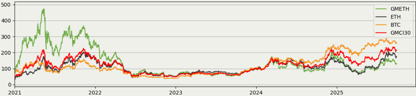
Performance GMETH vs GMCI30 vs BTC vs ETH
