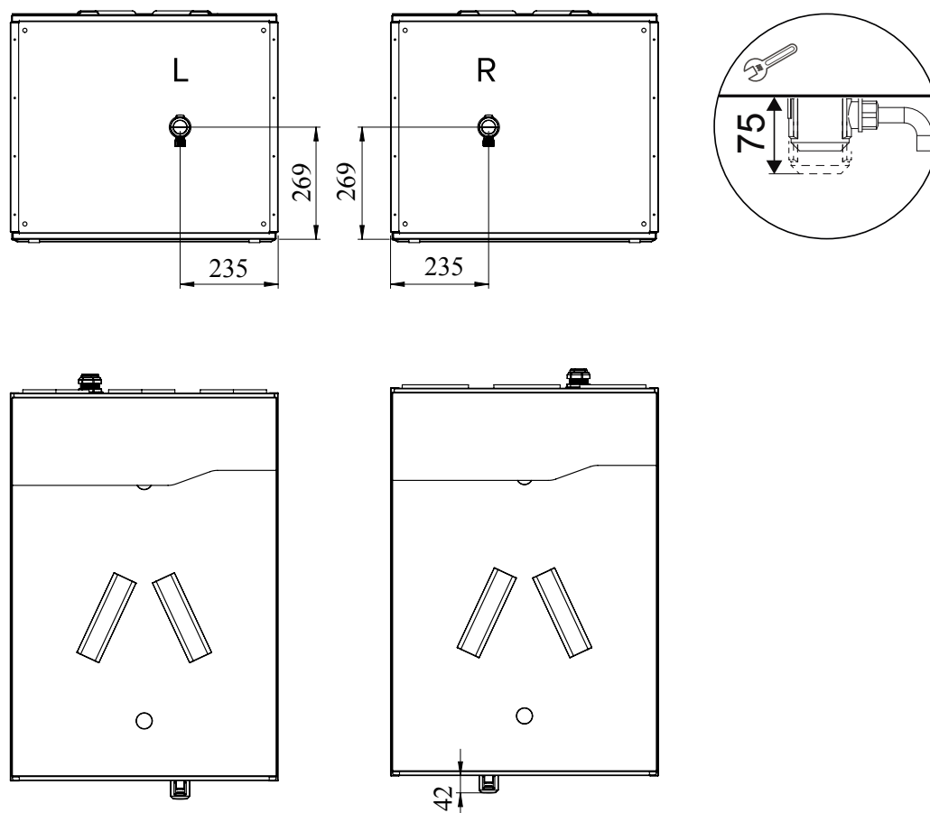
Figure 2. Space required by the alternative Vallox Silent Klick water seal installation method (elbow)
