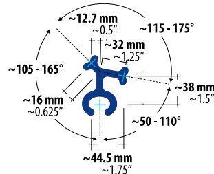
T connector
