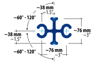
Cross connector
