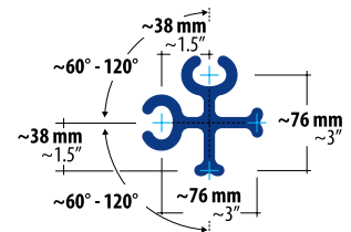
Cross connector
