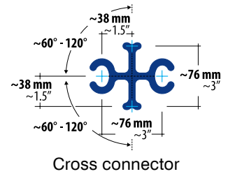
Cross connector
