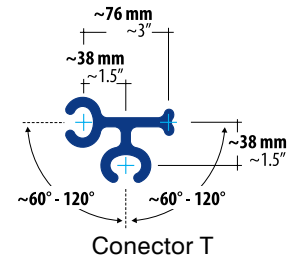
Conector T
