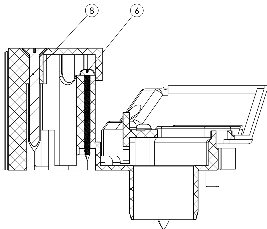
SECTION C-C
