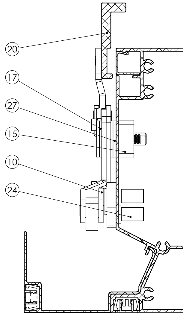
SECTION E-E
