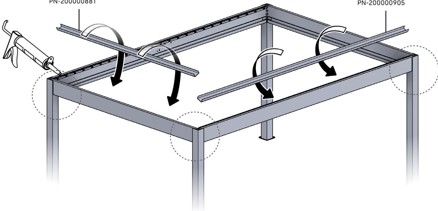
SKY GUTTER W BEAM FS 4M PN-200000881
