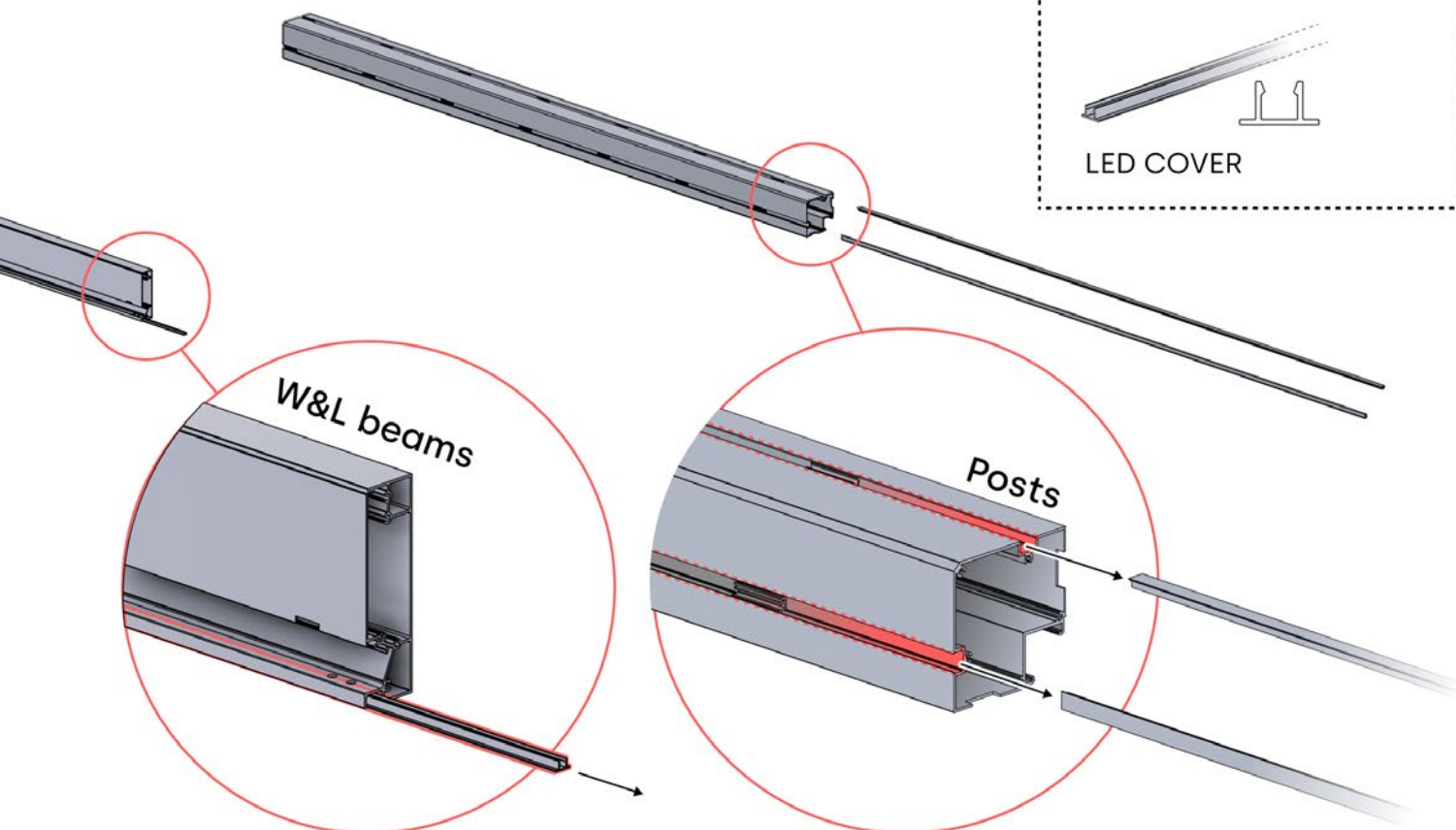
PN-200000512 LED STRIP COVER CLIP
