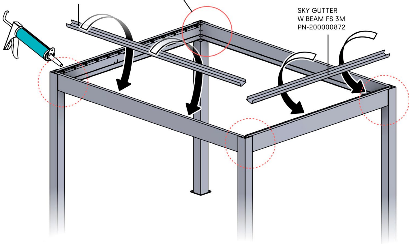
SKY GUTTER W BEAM FS 3M PN-200000872
