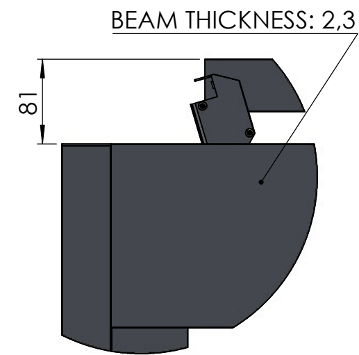
DETAIL A OPEN POSITION
