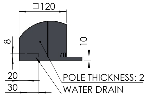
DETAIL B CORNER POLE
