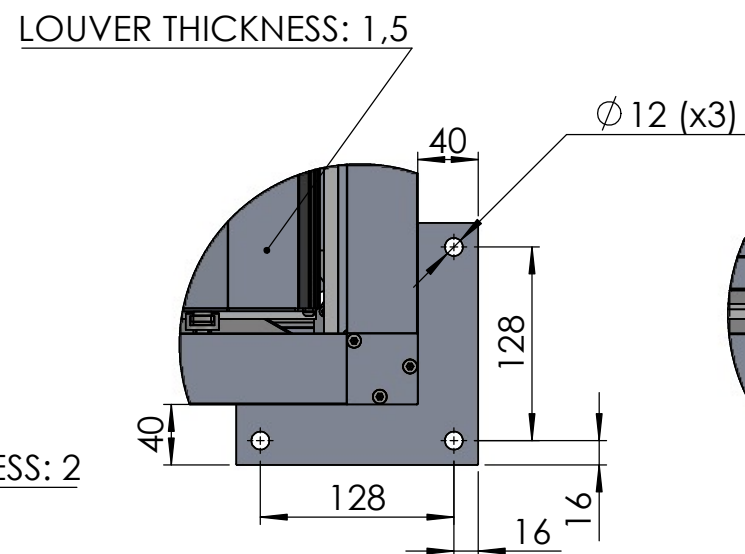
DETAIL C CORNER POLE
