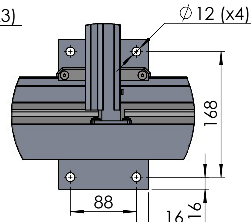
DETAIL D MIDDLE POLE
