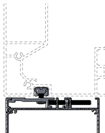
SECTION E-E
