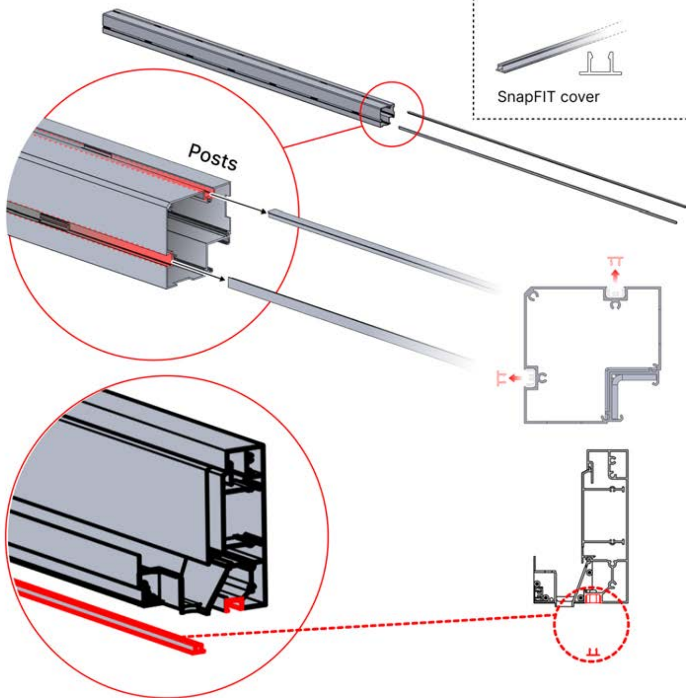
PN-200000512 SnapFIT cover clip
