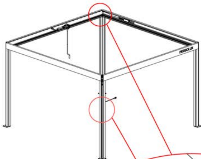
POWER CABLE
