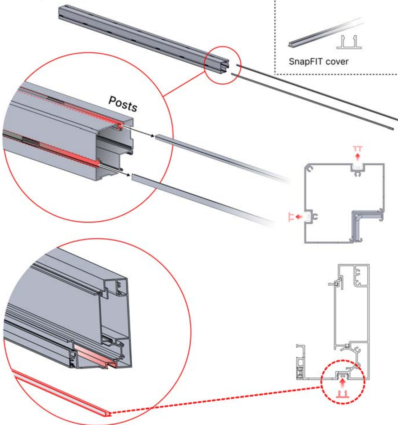
PN-200000512 SnapFIT cover clip
