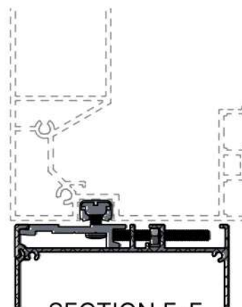
SECTION E-E
