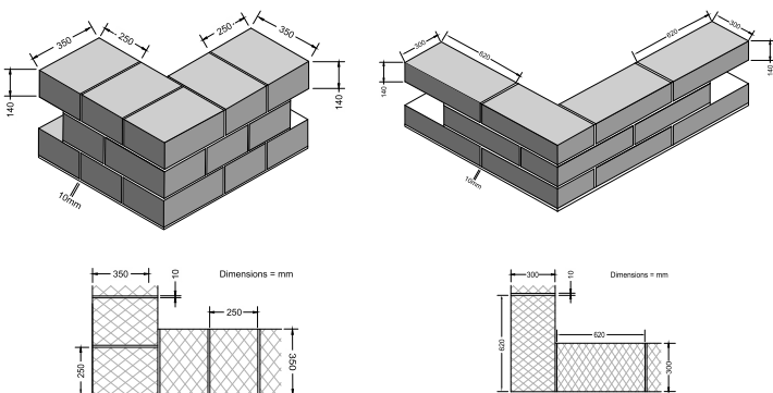
Example corner detail: 350 x 250 Armstart aggregate foundation block
