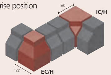
Kerb edging (low-rise position)
