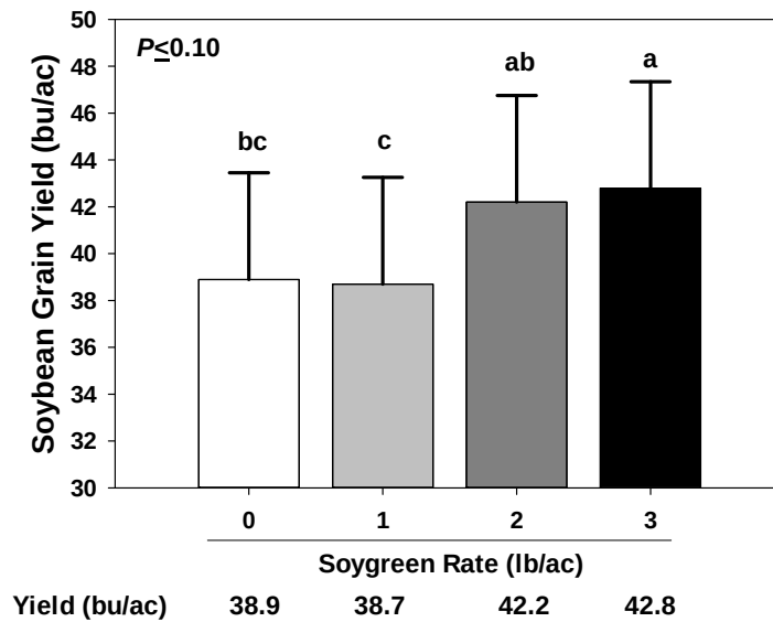
Fig. 4. Soybean grain yield response to 0, 1, 2 and 3 lb of Soygreen per acre applied directly on the soybean seed averaged across five locations in west-central Minnesota.
