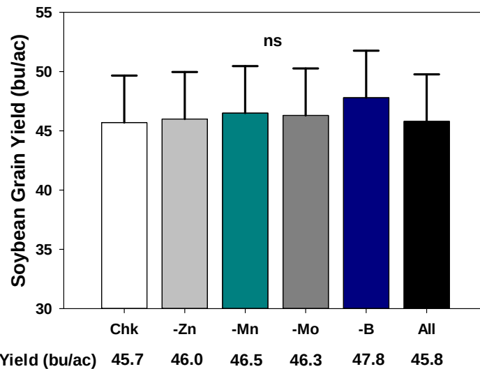
Fig. 6. Soybean grain yield of a non-fertilized control compared to the application of 10 lb of Zn, 10 lb. of Mn, 0.5 lb of Mo, and 2 lb of B broadcast and incorporated before planting and treatments where one of the micronutrients (-Zn, -Mn, -Mo, or -B) were omitted.
