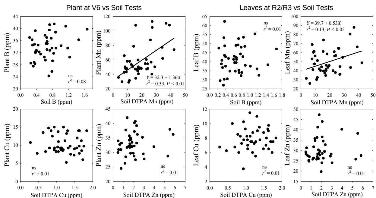
Fig. 2. Relationships across Iowa foliar fertilization trials between soybean tissue test results at two growth stages and soil-test results for B (hot-water test), Cu, Mn, and Zn(DTPA test).
