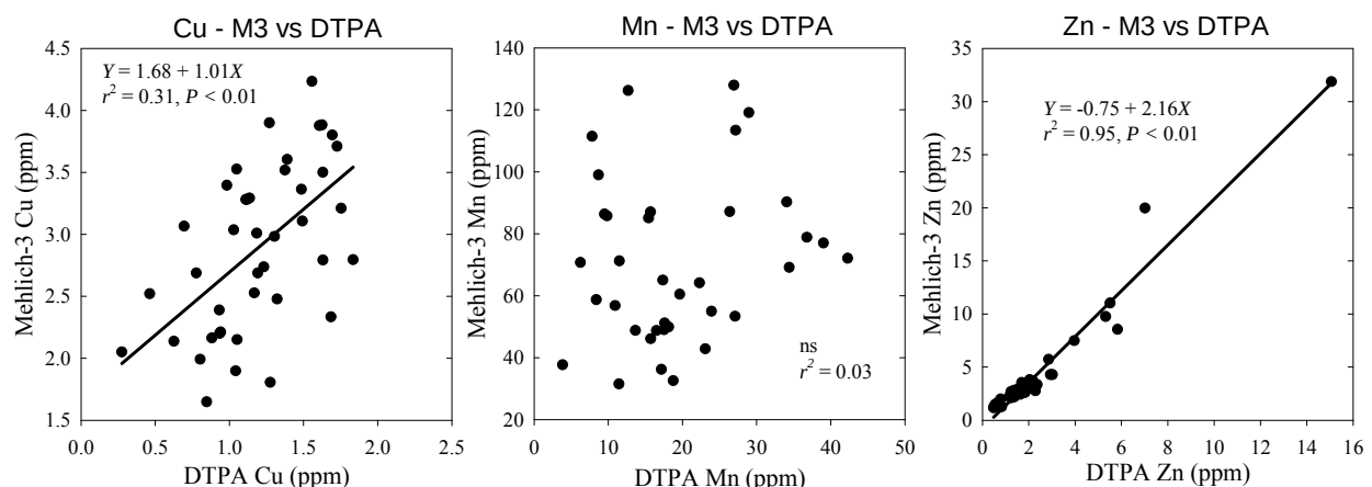
Fig. 1. Relationships across Iowa conventional plot trials soil Cu, Mn, and Zn measured with DTPA and Mehlich-3 test methods.
