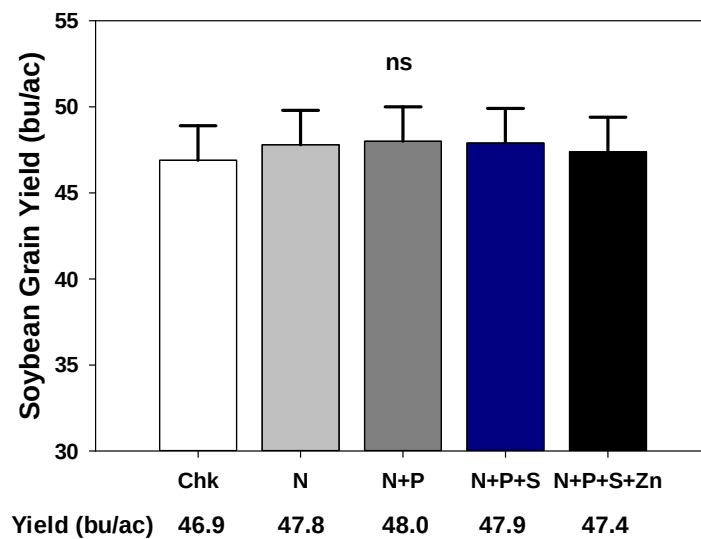
Fig. 5. Soybean grain yield response to 200 lb per acre of MicroEssentials-SZ broadcast before planting compared to a non-fertilized control and treatments that omitted one or more nutrients.
