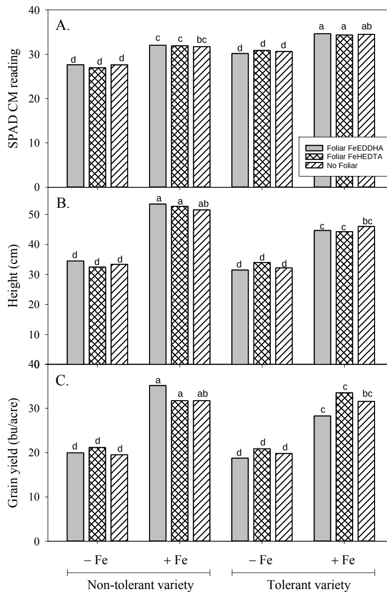
Fig. 3. Chlorophyll meter reading values, plant height and grain yield as affected by soybean variety selection seed-applied Fe-EDDHA – ortho- ortho fertilizer, and foliar applied chelated Fe (EDDHA and HEDTA). Average across seven site-years.
