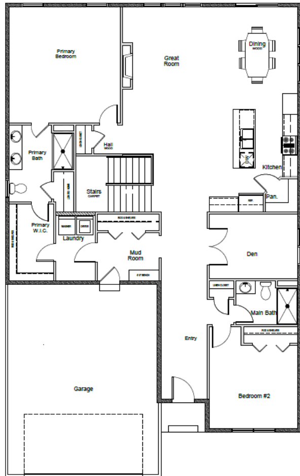
FIRST FLOOR PLAN SCALE: 1/8" = 1'-0"
