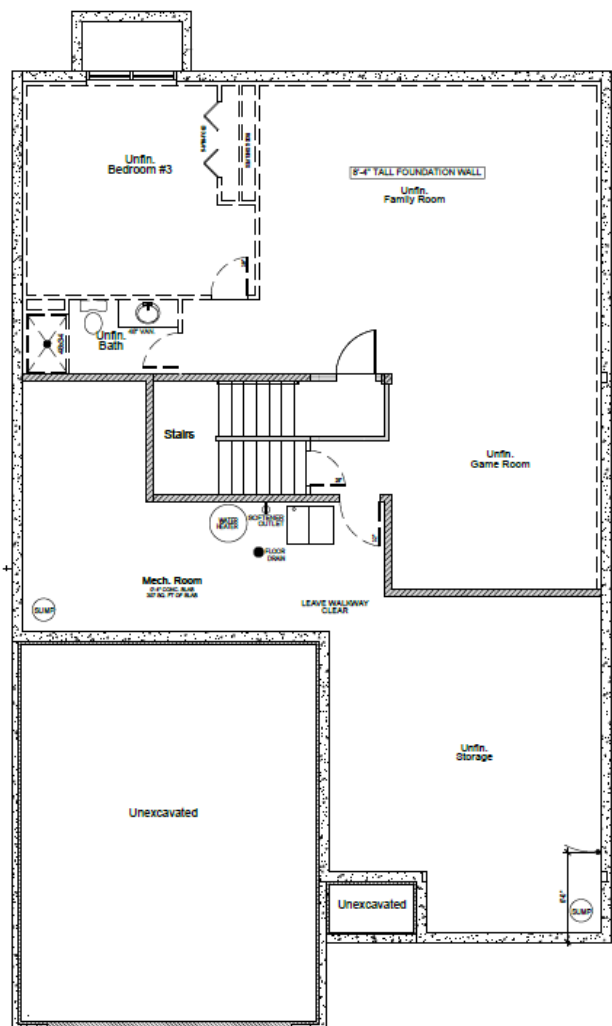
UNFINISHED BASEMENT FLOOR PLAN - FULL BASEMENT SCALE: 1/8" = 1'-0"
