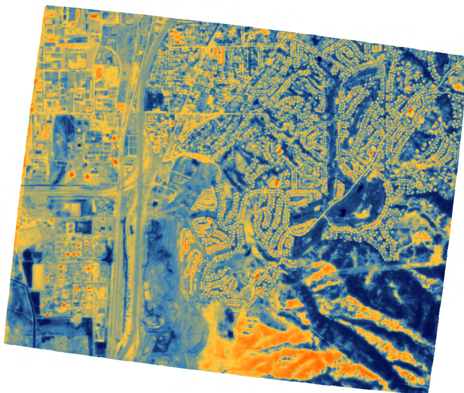
Figure 2. Surface Brightness Temperature scene showing enhanced signal to noise characteristics over a single primary frame, orthorectified and projected onto an elevation model
