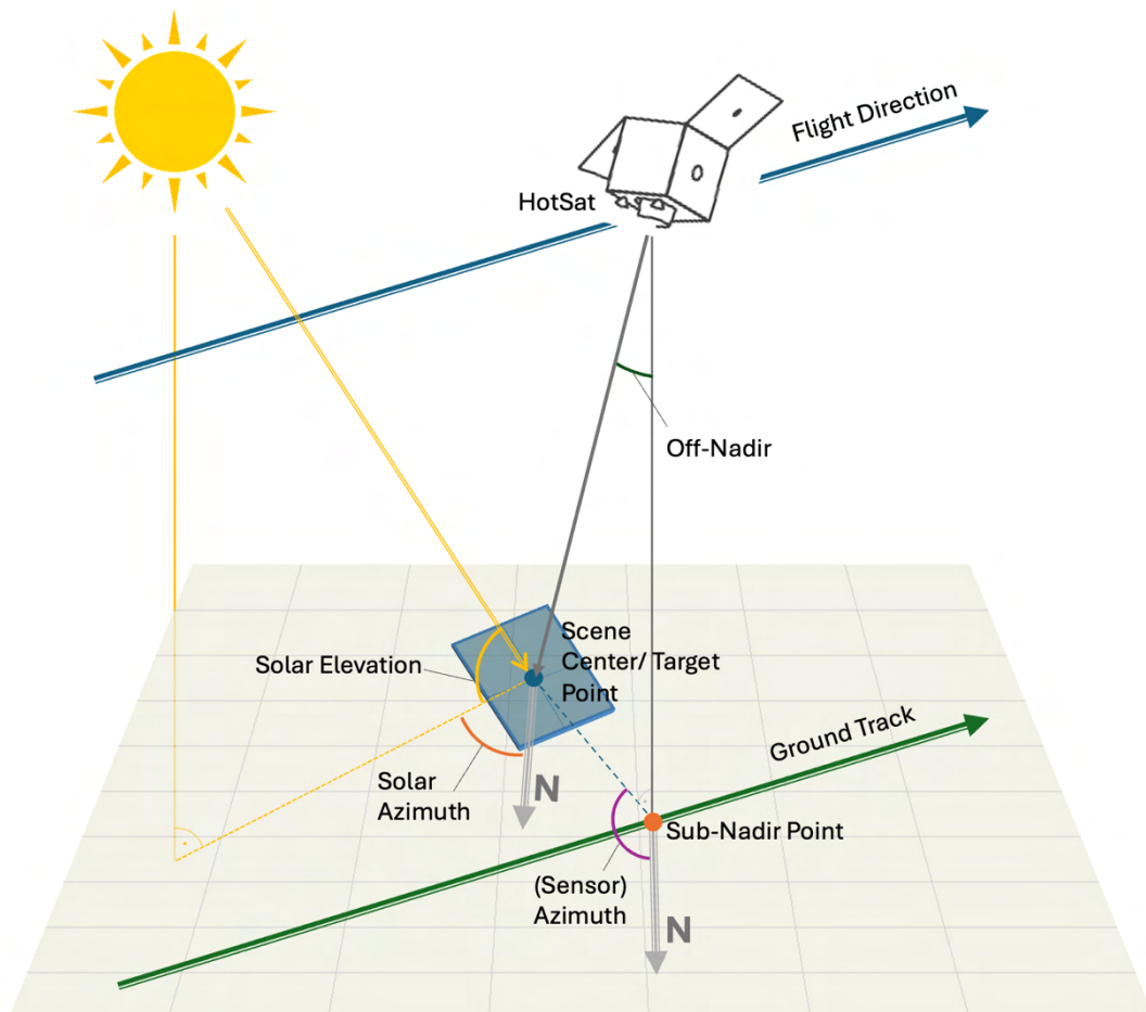
Figure 8 Sensor viewing geometry
