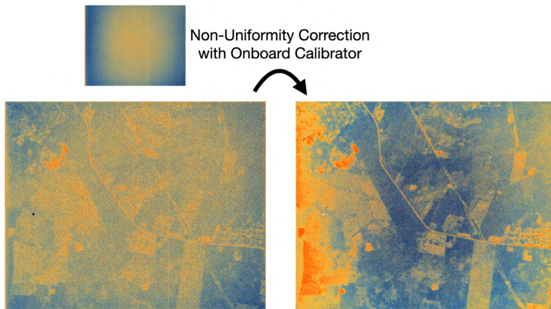
Figure 6. Applying non-uniformity correction
