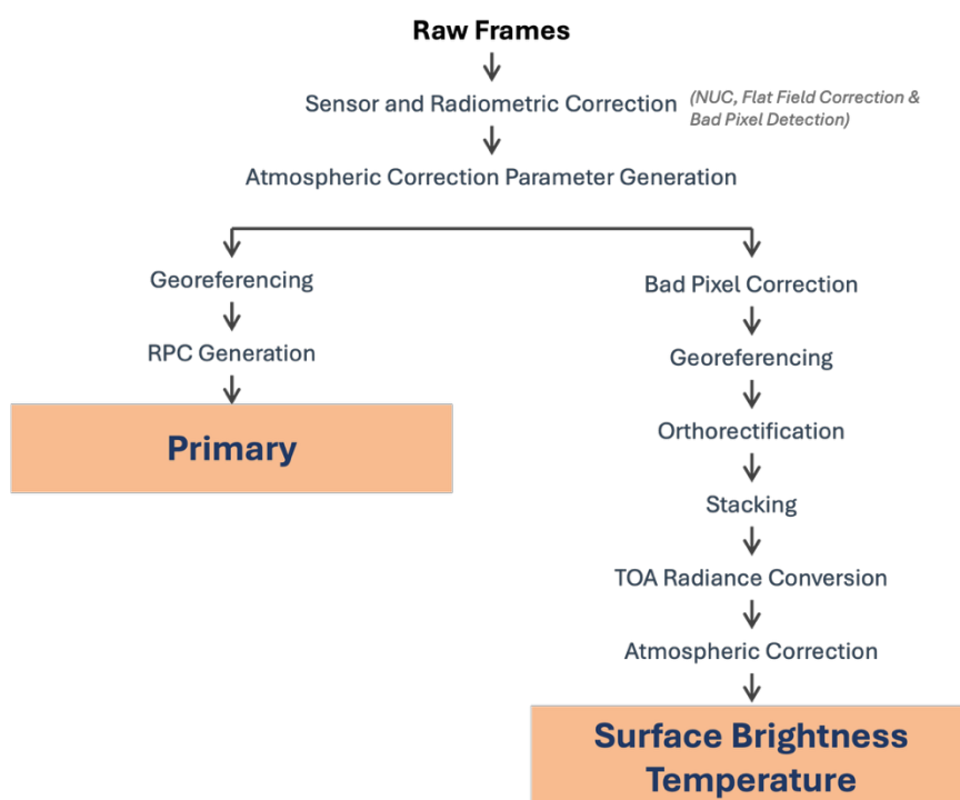
Figure 3. Image Processing workflow
