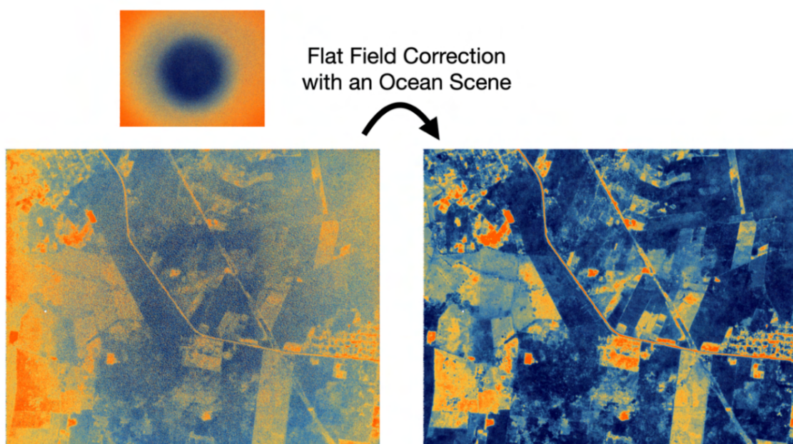
Figure 7. Applying flat field correction
