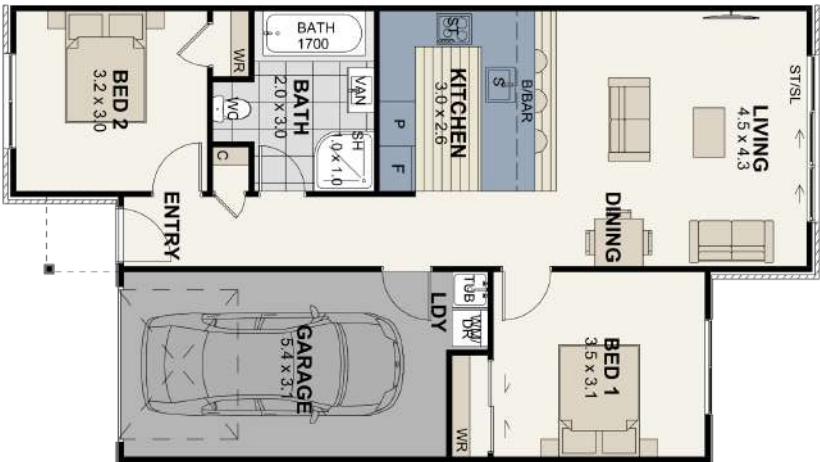
Floor Plan
