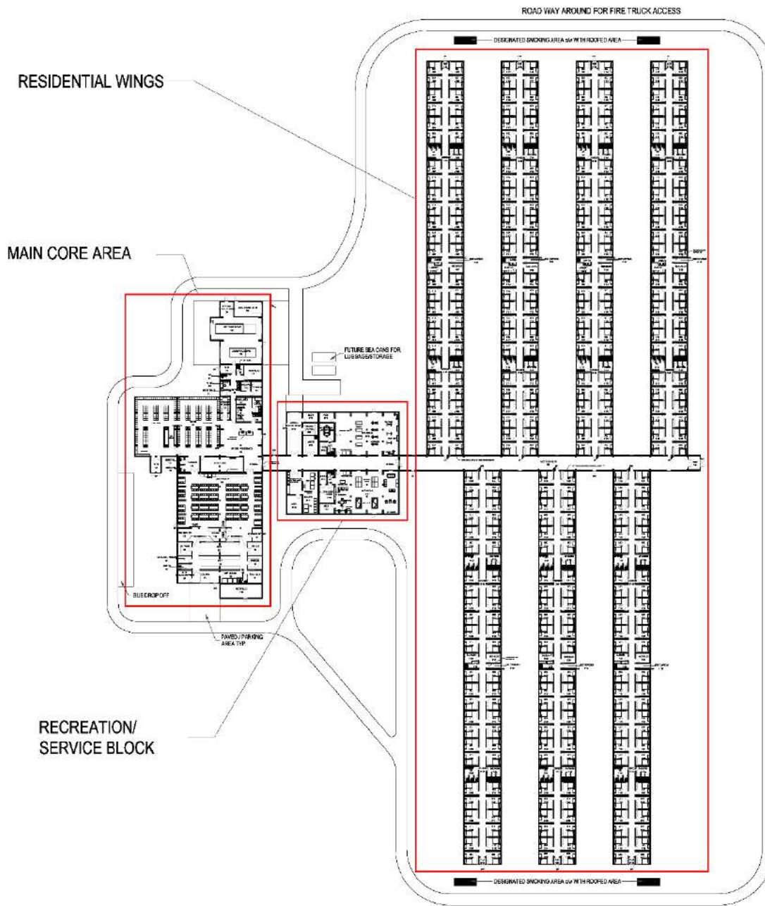
Figure 18-2: Camp Layout
