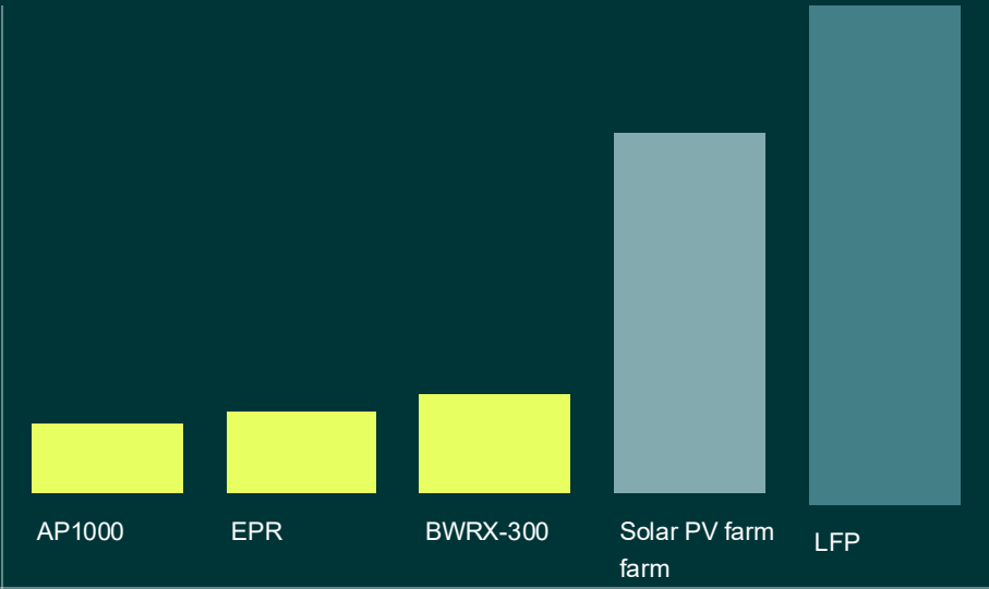
Kg OF ROCK PER GWh GENERATION CLEAN ELECTRICITY GENERATION SOURCE
