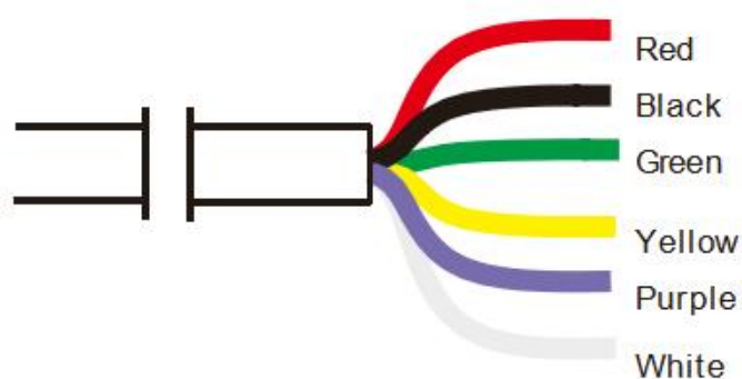
Figure 1 Cable Diagram
