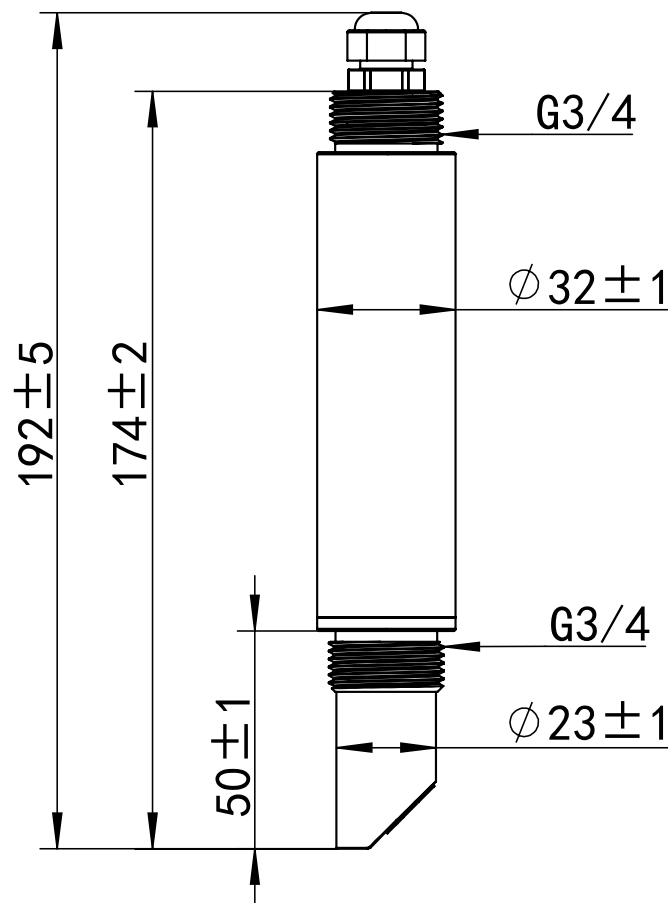
Figure 2 Dimensions (Unit: mm)
