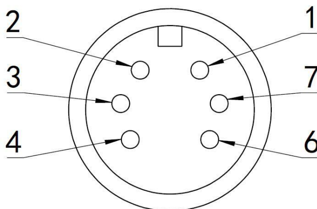
Figure 2 Cable Diagram
