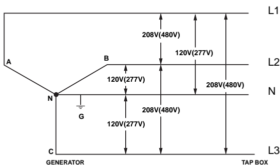
Low (High) - Wye Connection
