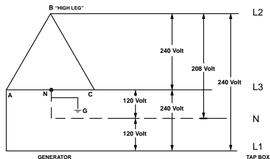
Delta 4-Wire Connection [Delta 3-Wire eliminates Neutral (N) connection (dashed line)]
