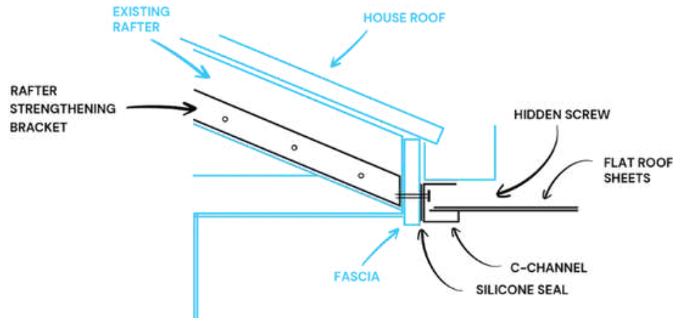
Attached to fascia
