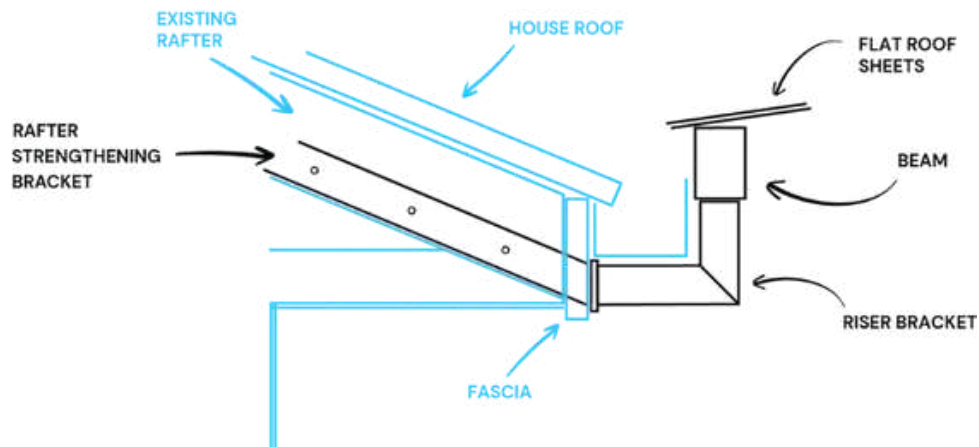
Attached to riser brackets
