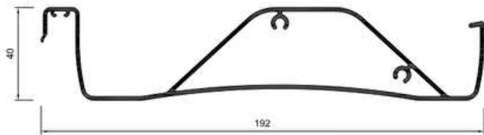
Louvre blade profile
