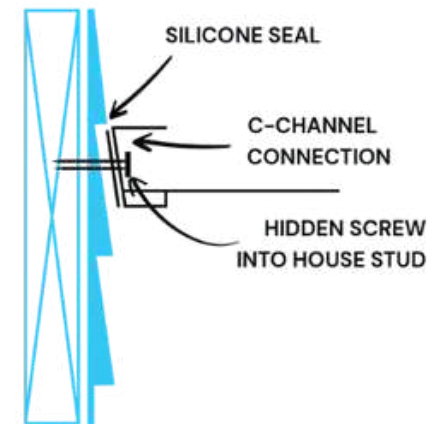
Wall-fixed to weatherboards
