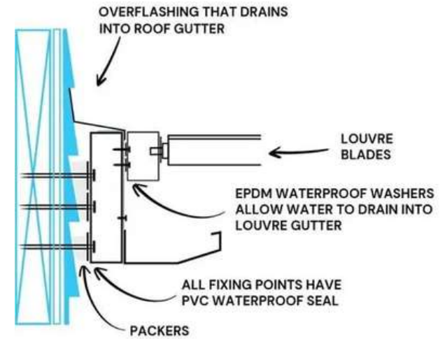
Wall-fixed to cladding or brick
