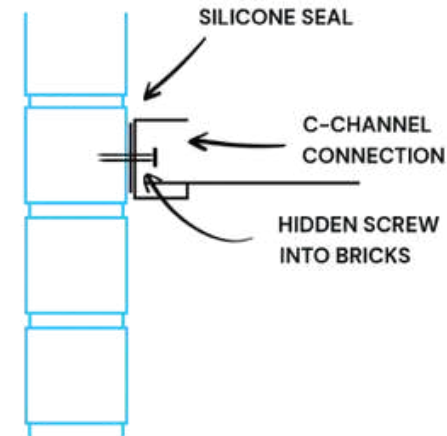
Wall-fixed to brick
