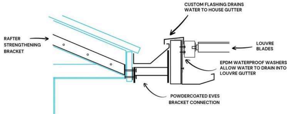
Attached to fascia
