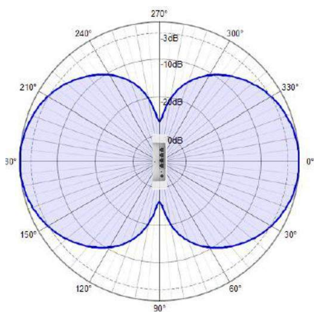
Radiation Pattern (Vertical)
