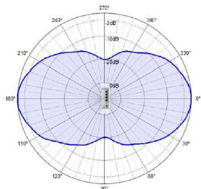
Radiation Pattern (Vertical)
