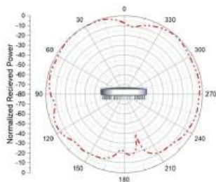
Radiation Pattern (Vertical)
