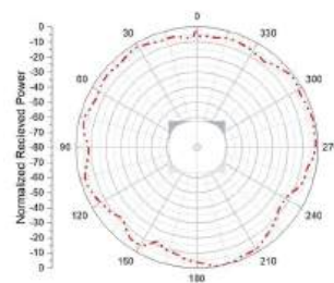
Radiation Pattern (Horizontal)
