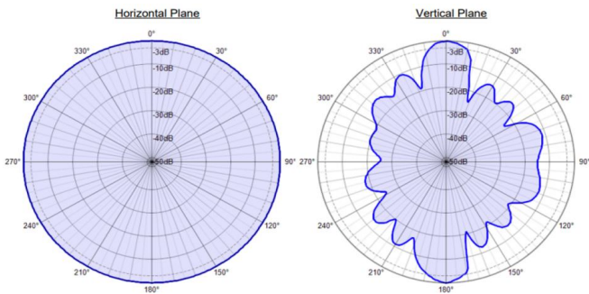
Radiation Pattern 2450 MHz
