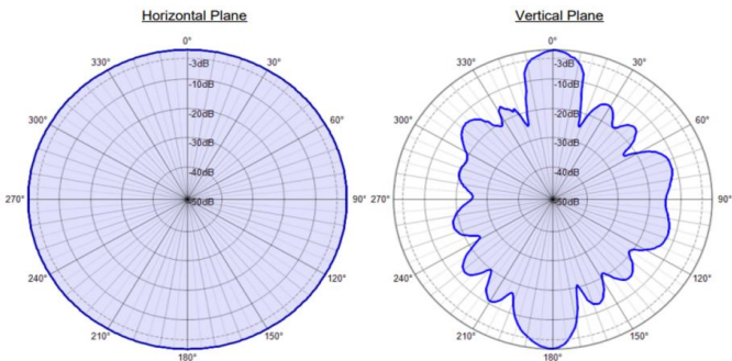
Radiation Pattern 5500 MHz
