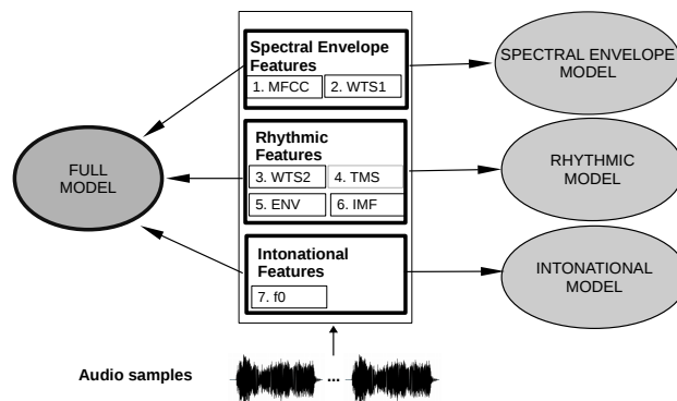
Figure 1: Figure 1: Acoustic measures derived from audio samples: 1. The mel-frequency cepstral coefficients (MFCC) are cepstral representations of the audio sample that concisely describe the overall shape of a spectral envelope as perceived by human. MFCC features were taken as the average of 13 coefficients derived using a 40-band filter bank (133-6864 Hz) on hamming windows of 500ms, each overlapping for 250ms; 2 & 3. The wavelet time scattering (WTS) transform represents low-variance time-frequency properties that capture the spectral envelope of sounds related to segmental features (WTS1), and larger-scale structures like amplitude and frequency modulations relevant to rhythm (WTS2). WT1 and WTS2 were taken as averages of log-transformed scattering features, respectively computed using a first wavelet filter bank with 8 wavelets per octave, and a second wavelet filter bank with one wavelet per octave, over non-overlapping windows of 1 sec; 4. The temporal modulation spectrum (TMS) is the frequency decomposition of the temporal envelope of a signal that is a primary acoustic correlate of perceived rhythm in speech, derived using the method described in Ding et al. (2017); 5 & 6. The speech envelope spectrum (ENV) represents temporal regularities correlating to rhythmic properties. Intrinsic mode functions (IMF) were decompositions of the ENV using empirical mode decomposition. IMFs represent time-scales of oscillation in the envelope that reflect both syllable-driven and prosodic-feet-level fluctuations. ENV and IMF were derived using the methods described in Tilsen and Arvaniti (2013); 7. The f0 contour is a major acoustic correlate of pitch melody and speech intonation, derived from taking 20 f0 values from the raw f0 contour taken at equal proportional intervals. Further, spectral envelope (MFCC and WTS1), rhythmic (ENV, IMF, WTS2, and TMS), and intonational (f0) acoustic measures were input in combination to the Full Model, and individually into respective models corresponding to the three classes of acoustic measures.
