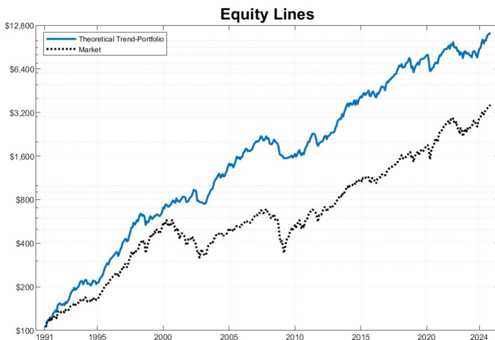
Figure 13: A comparison between the Theoretical Trend Portfolio (blue line) and a market capitalization-weighted index of all US stocks (black line). Theoretical refers to the fact that this version of the strategy does not account for transaction costs, slippage, or interest, and it also allows for trading of fractional shares.
