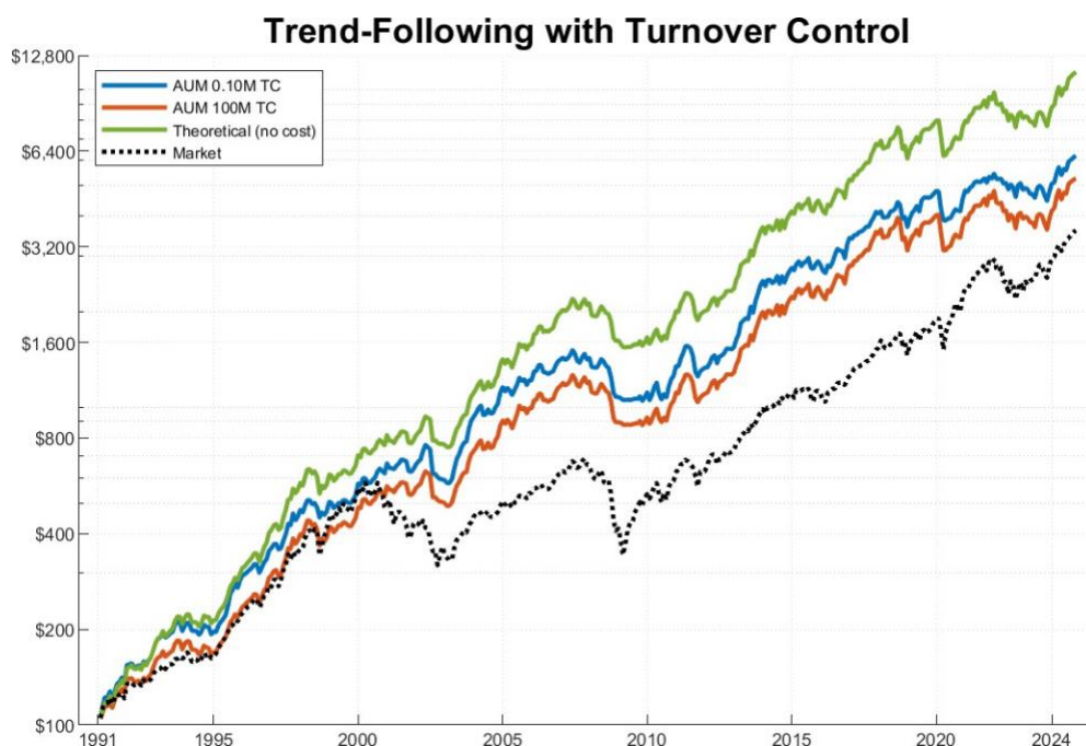
Figure 20: NAV comparison between the Theoretical Trend Portfolio (green line) and two historically accurate backtests with AUM sizes of 0.1M and 100M. While AUM is artificially reset at the beginning of each year, NAV remains unaffected. These backtests account for realistic trading cost assumptions, as detailed in Section 4.7, and incorporate the turnover control mechanism described in Section 4.8. The black dotted line represents a market capitalization-weighted index of all U.S. stocks.
