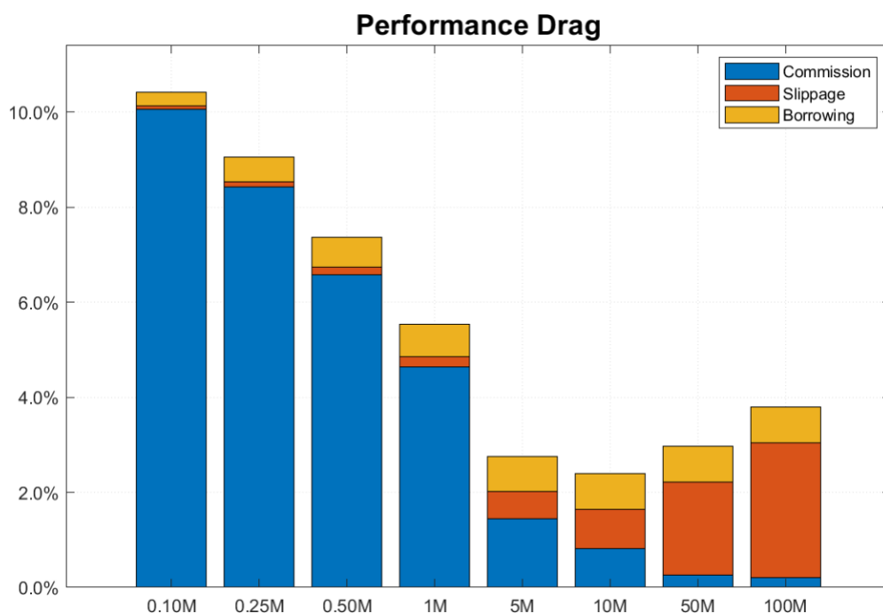
Figure 17: This vertical stacked bar chart illustrates the impact of realistic trading costs on eight trend-following portfolios with varying AUM sizes (ranging from 0.10M to 100M). The stacked bars represent the average yearly impact of commissions (blue), slippage (orange), and borrowing costs (yellow), expressed as a percentage of the portfolio's AUM.
