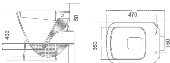
P TRAP
