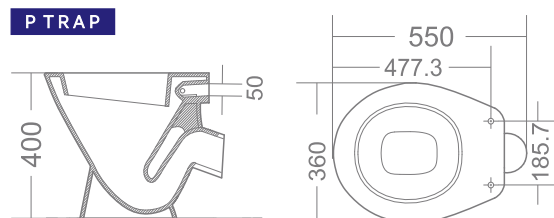
P TRAP
