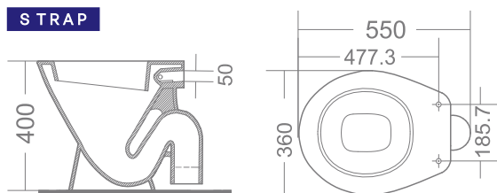
S TRAP
