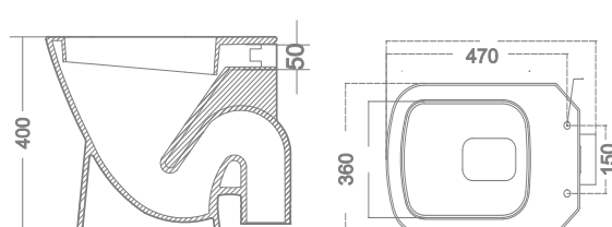
S TRAP
