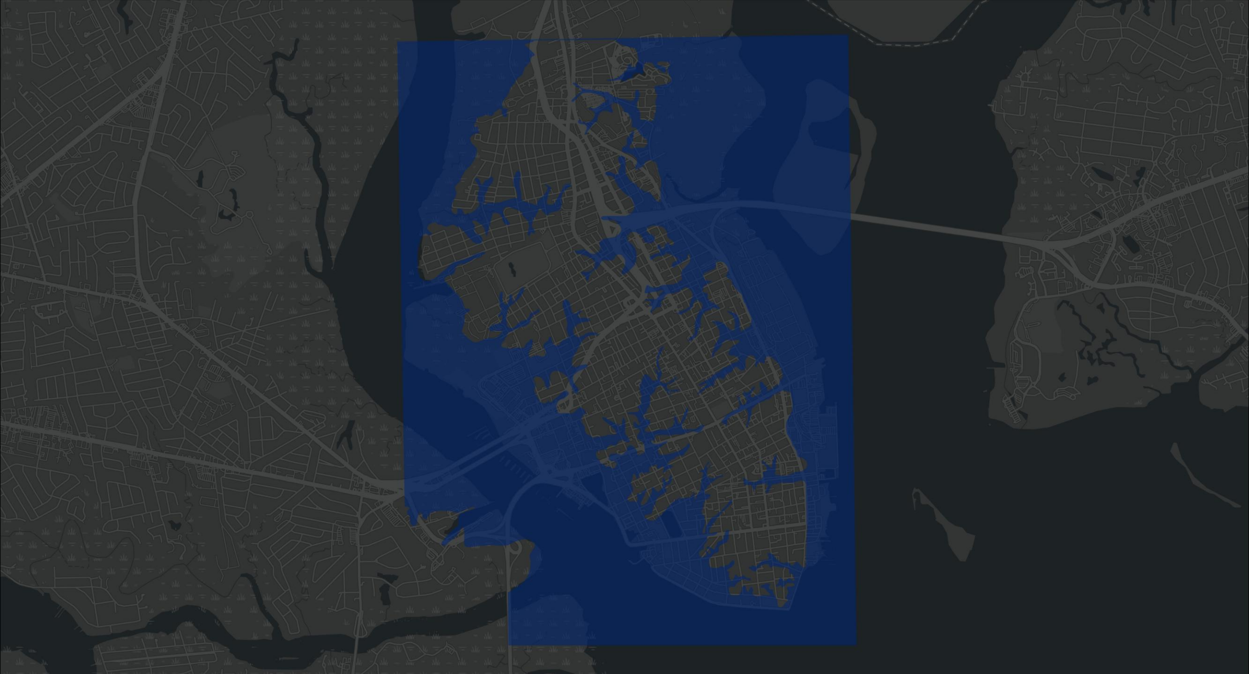
Historic Tidal Creeks overlaid on the Peninsula
