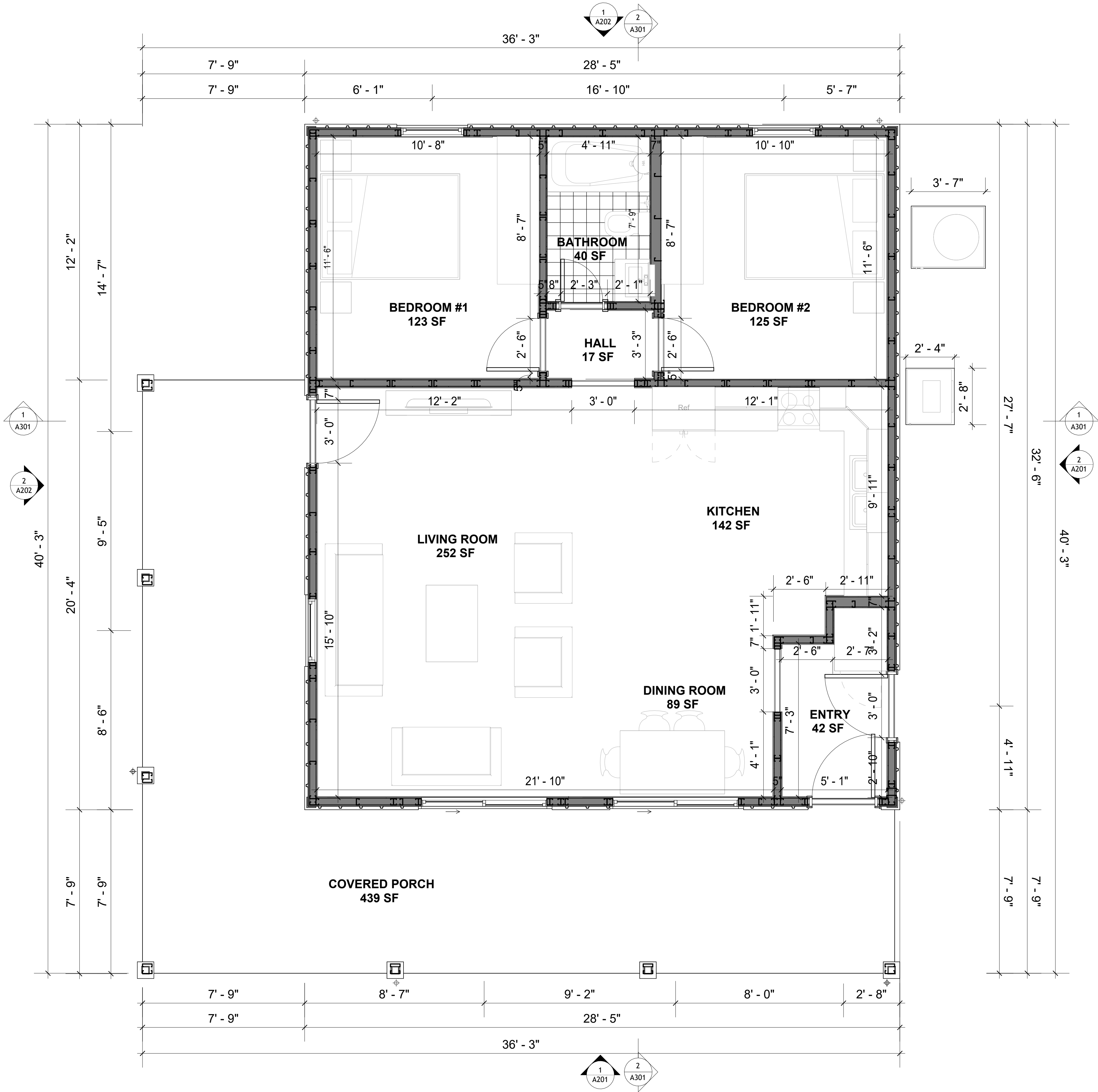
1 DIMENSION PLAN 3/8" = 1'-0"
