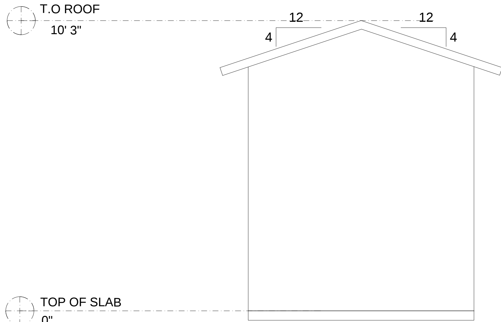
Front Elevation
