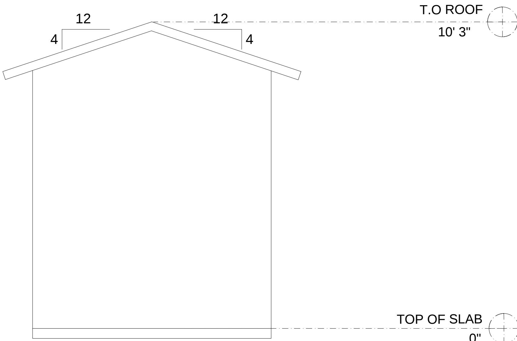
Rear Elevation
