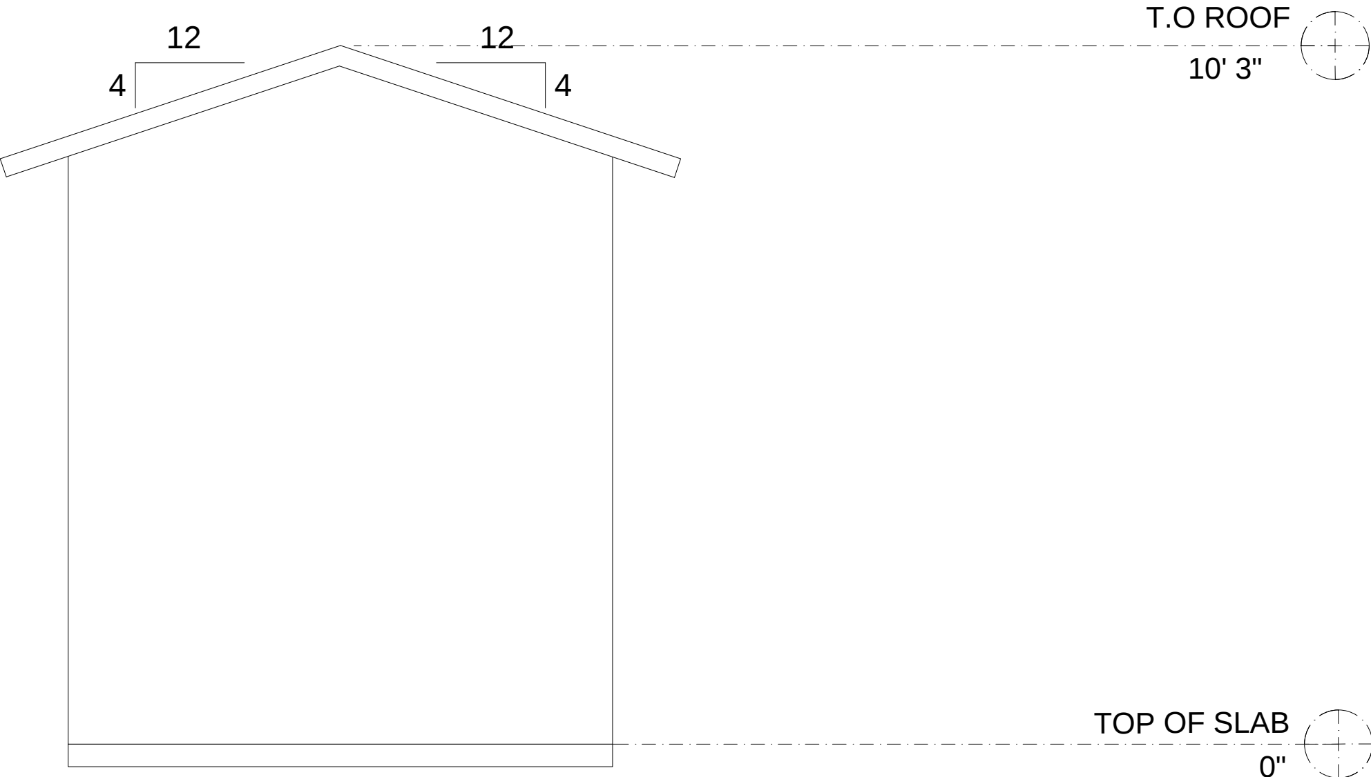
Rear Elevation
