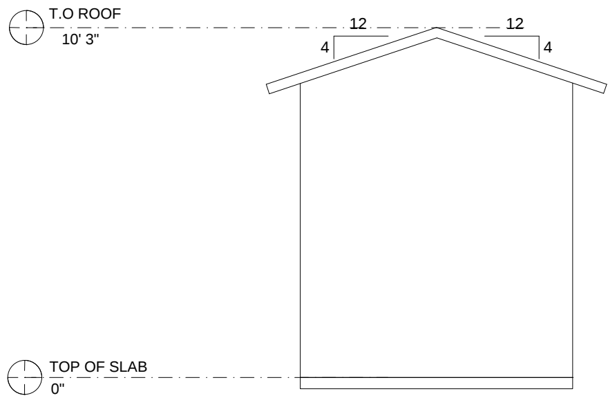
Front Elevation
