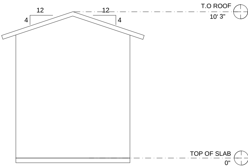
Rear Elevation
