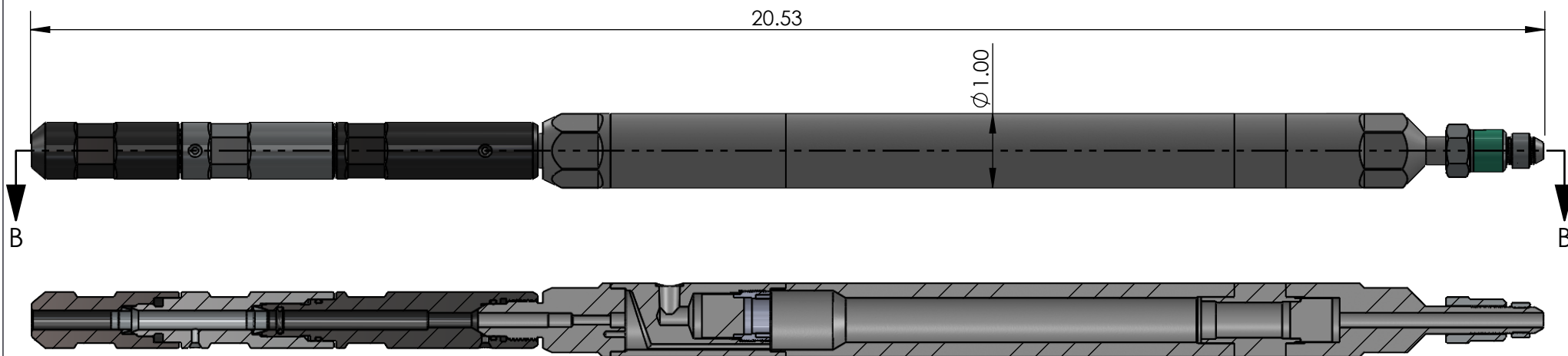
SECTION B-B
