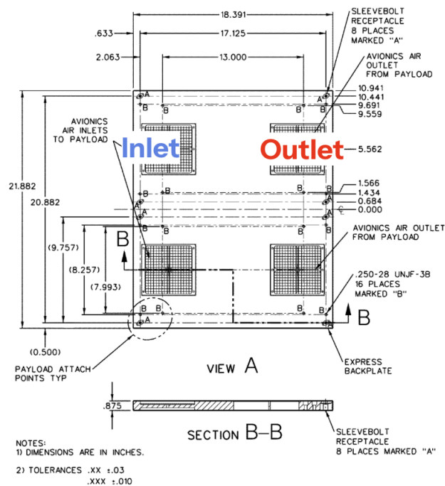
FIGURE 5. BACKPLATE INTERFACE (SSP 57000 FIGURE 3.2.1-3) (FRONT VIEW)
