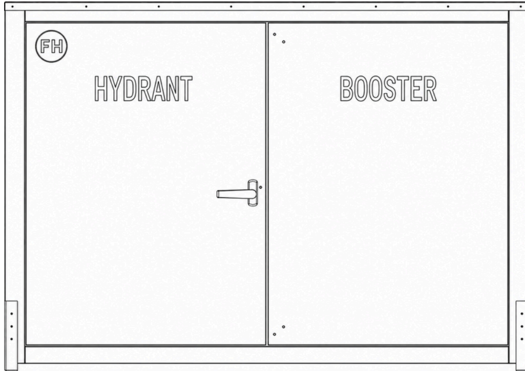
Front Elevation - Hydrant & Booster Cabinet
