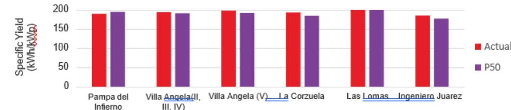
February Specific Generation Results: Actual vs P50. Source: CAMMESA and MSU EYA Reports.
