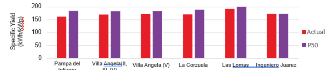
March Specific Generation Results: Actual vs P50. Source: CAMMESA and MSU EYA Reports.
