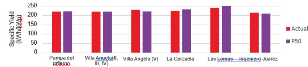
January Specific Generation Results: Actual vs P50. Source: CAMMESA and MSU EYA Reports.
