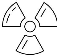
Radioactive Elements
