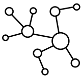
Protein
