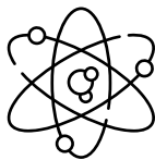
Atom
