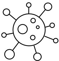
Virus
