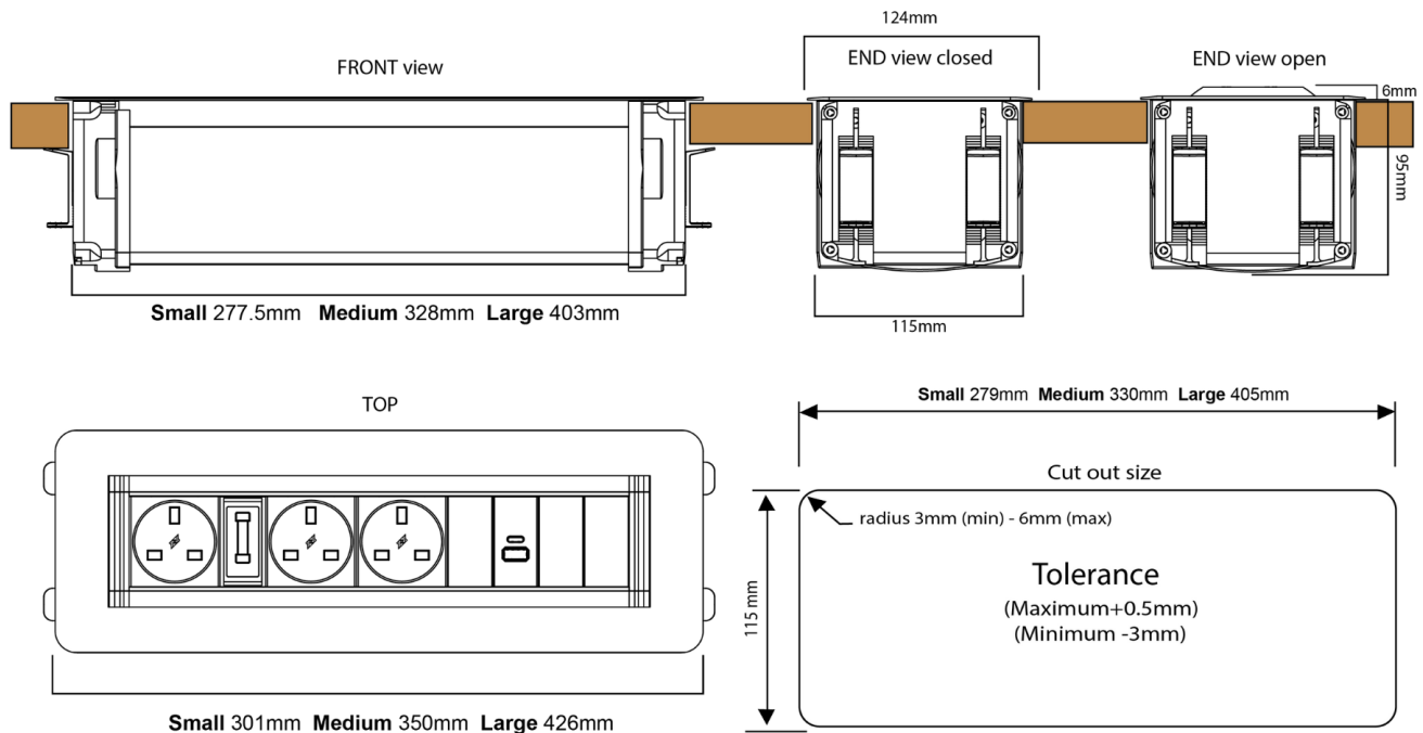
Technical dimension sketch (front / end / top / cut-out)
