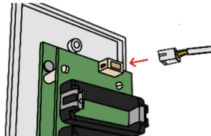
Connection of tether to the FXI Device
