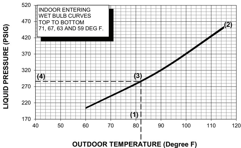
Figure 37. Pressure curves - model 5TTR4018A1
